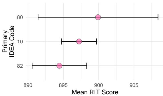
Math High School
