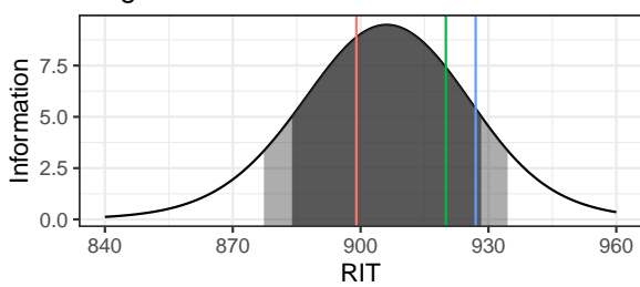
Math: High School
