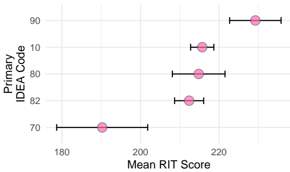
ELA High School
