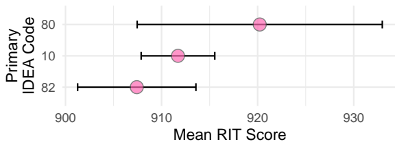
Science High School
