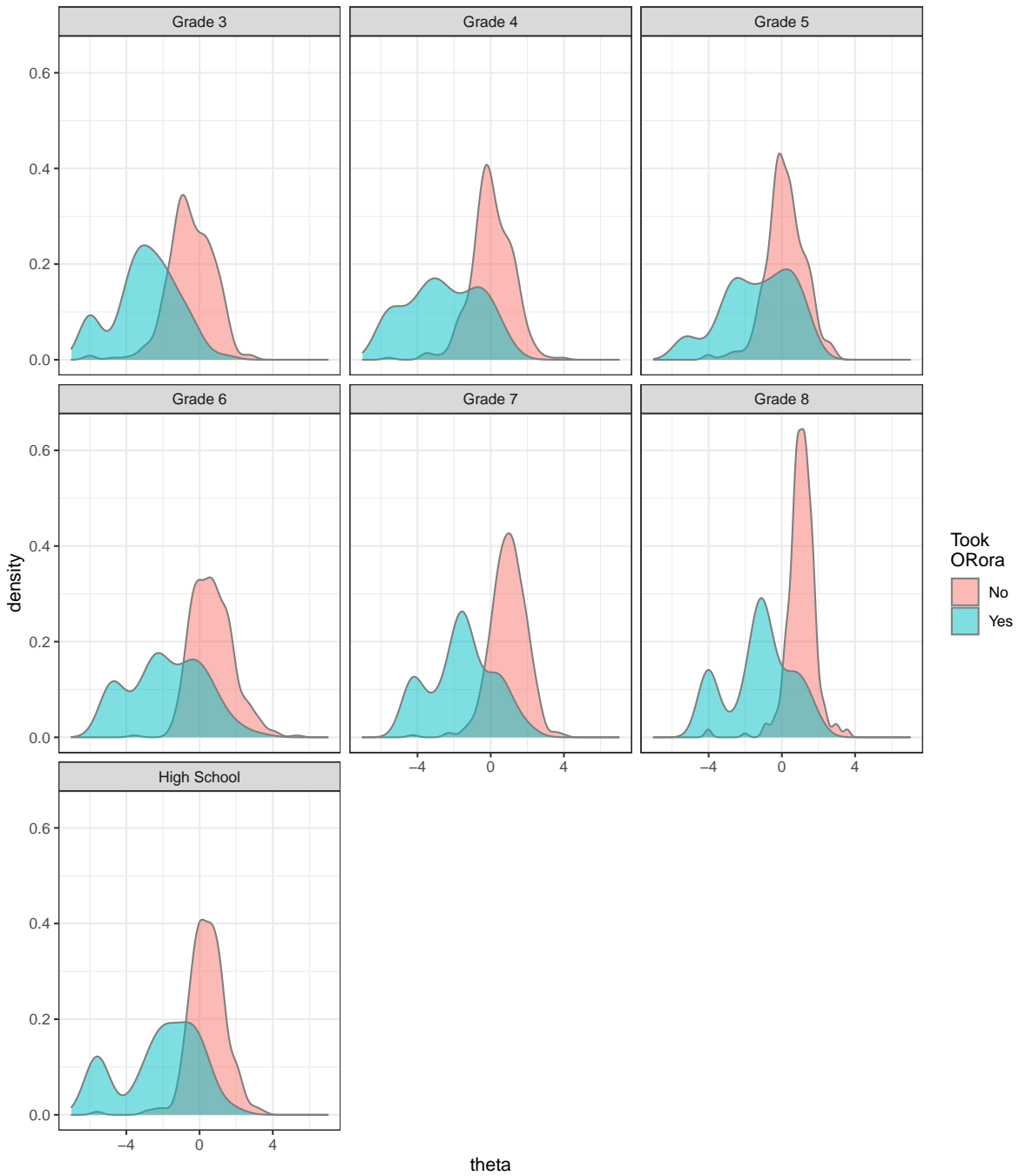
Math ability estimates (theta) for those who did vs. not take the ORora, by grade
